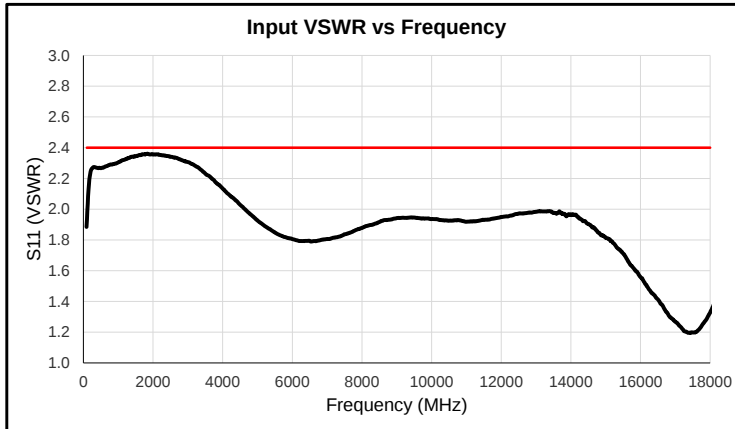
Typical Performance @ 23°C (Reference S/N 2162275)
